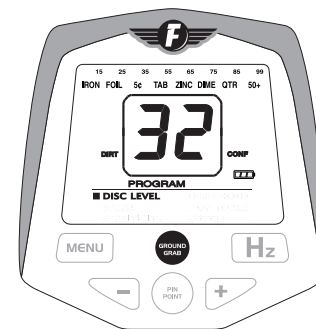
The detector will not balance in DISCRIMINATION mode where the GROUND PHASE is less than 40
