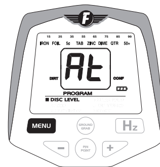
If the ground reads less than 40, enter AUTOTUNE mode (see Menu System pg. 12)
